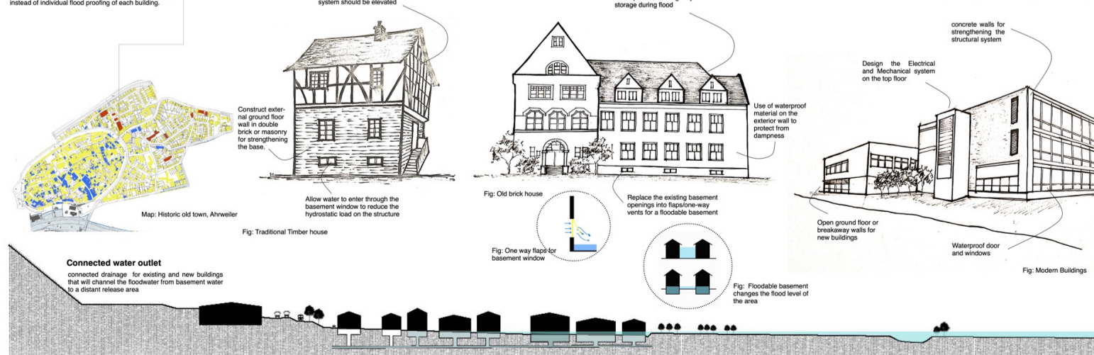
Floodgates The old town of Ahrweiler is surrounded by thick wall and a trench inside. This area contains the traditional Timber houses which are located densely. In this area, a common measure such as use of Floodgates is preferable instead of individual flood proofing of each building.
